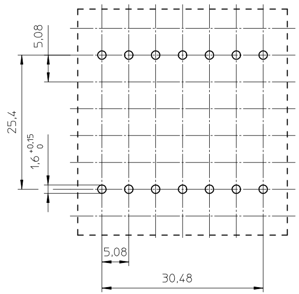
HOLE PATTERN:
